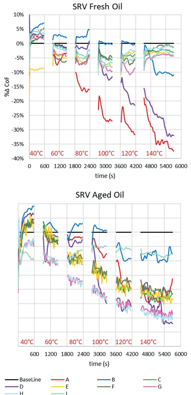
Figure 6: SRV friction profile relative to baseline formula 00.
